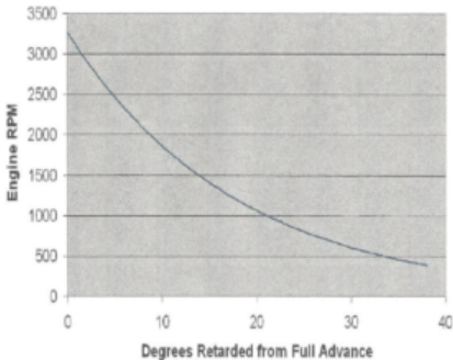
Typical Twin Ignition Curve MK2
